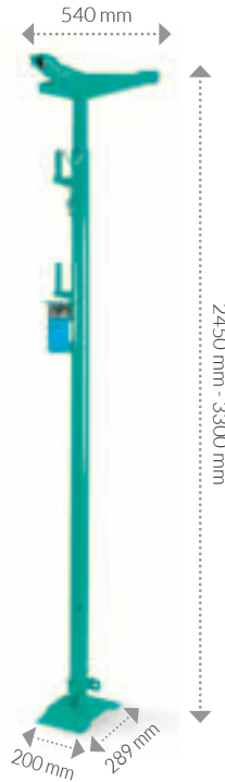
[ B ] Internal adjustable prop (2.45 m to 3.3 m) For using the hoists indoors or where there are no external scaffolding structures; height adjustable from a min. of 2.45 m to a max. of 3.3 m.
